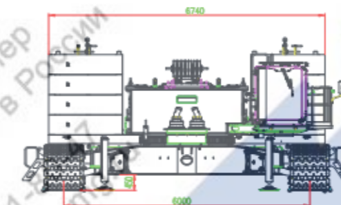
Outline drawing of XLC150 crawler crane
