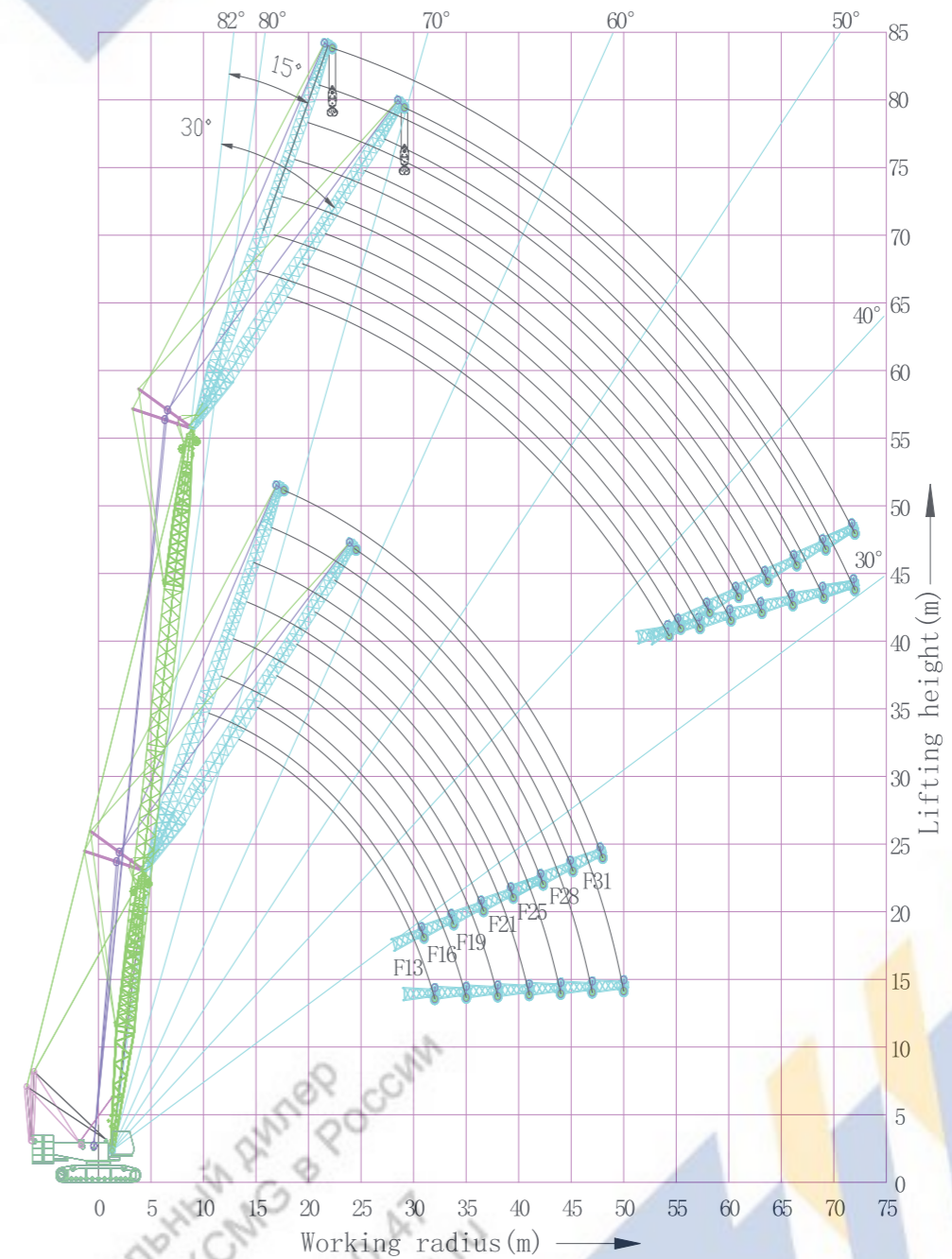
2.4 Working radius under fixed jib working condition ( HF )
